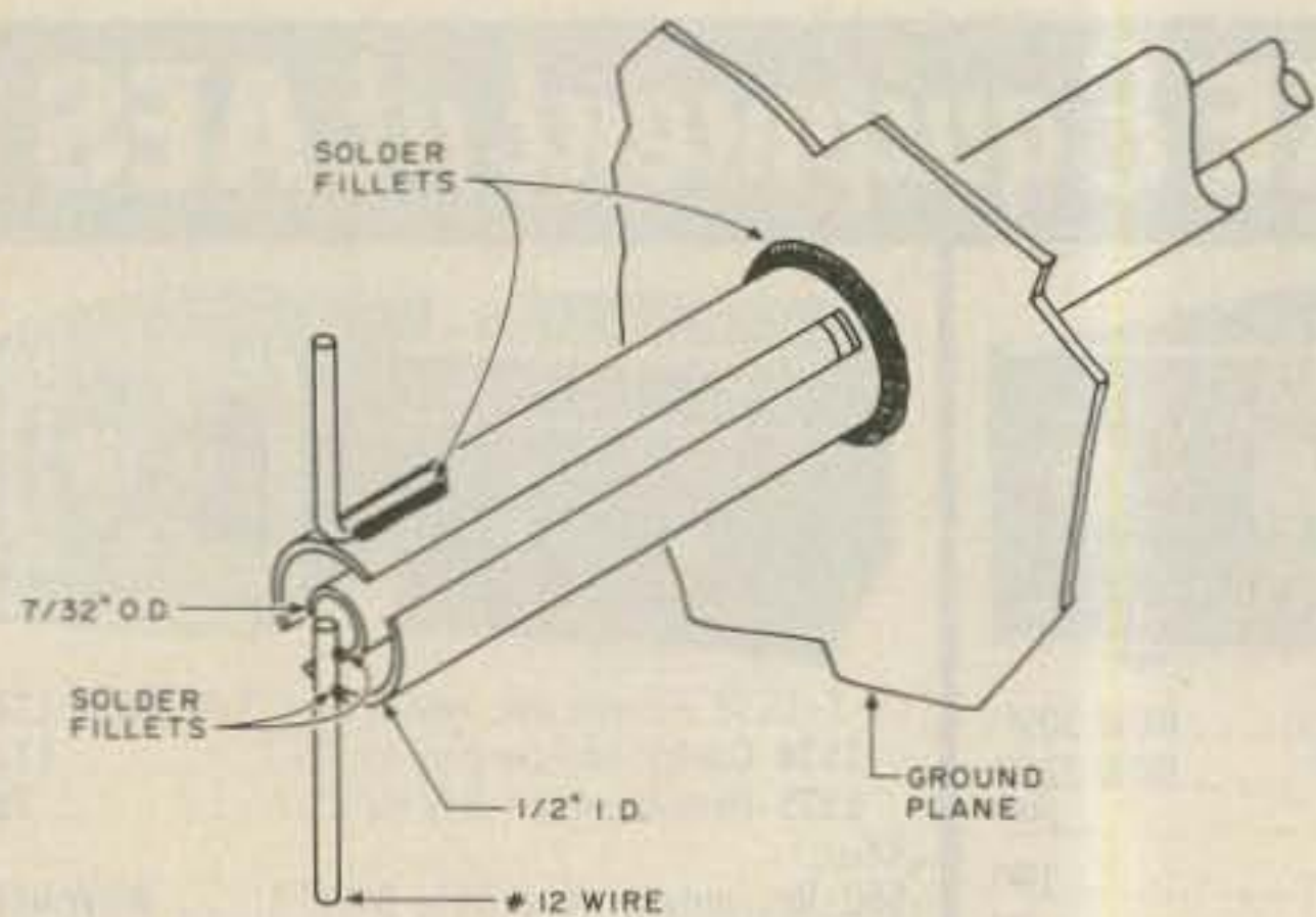
Fig. 2. Dipole-feed details.
