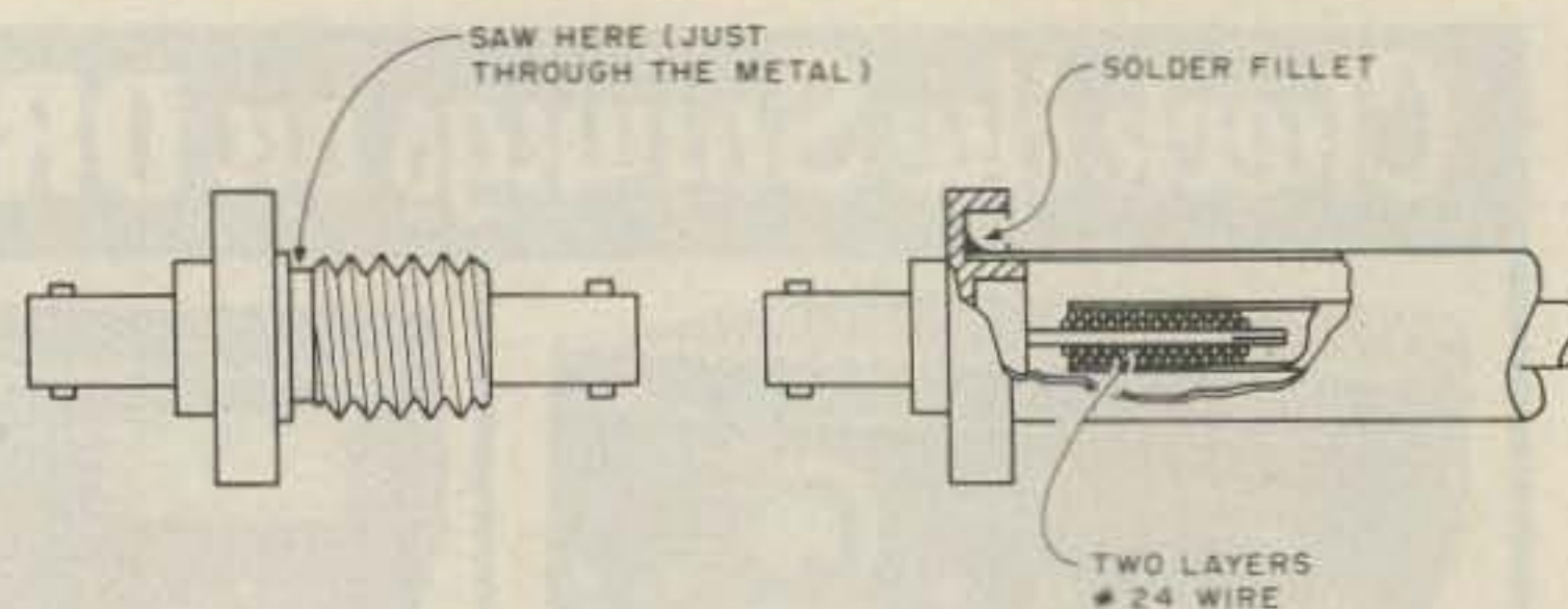
Fig. 3. Connector details.
